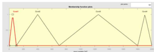
Fig 3. Hydrogen (H2) membership Function
