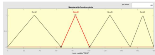
Fig 7. C2H6 membership Function
