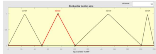
Fig 6. C2H4 membership Function
