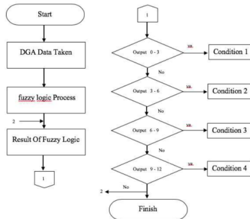
Fig 2. System Flowchart
