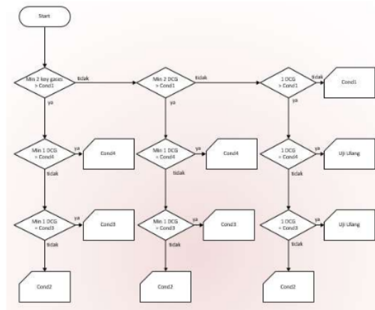
Fig 1. DGA Testing Flowchart[2]
