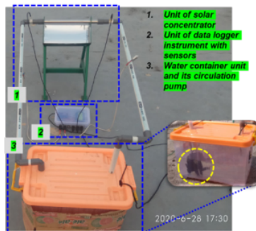
Figure 1 The main parts of a solar concentrator.
