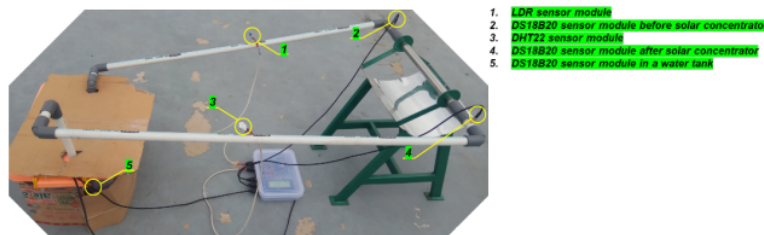
Figure 3 Measuring points in the solar concentrator.
